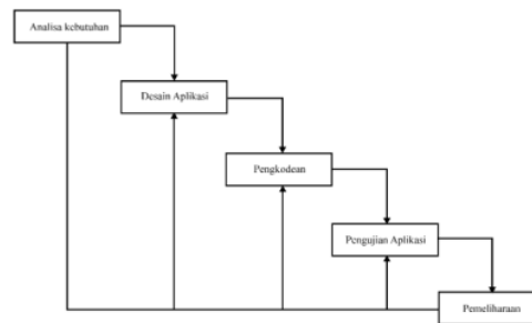
Gambar 2 Metode Waterfall
