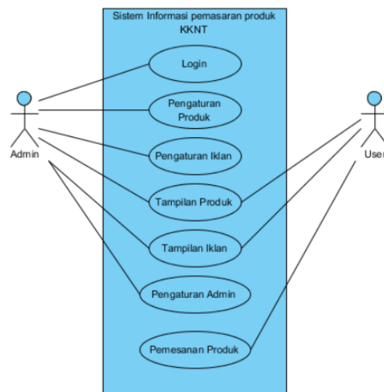
Gambar 3 Use Case.
